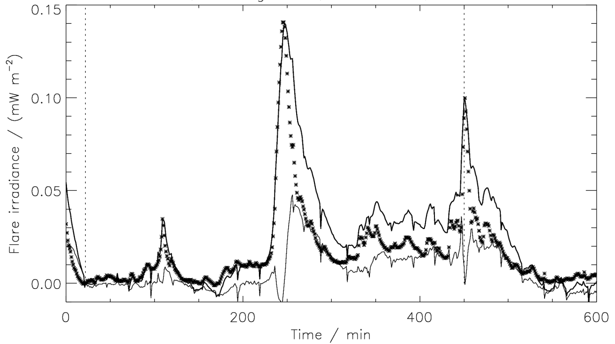
C1.3 flare, 08 Aug 2012, 07:31 UTC, ch3-120*SXR
