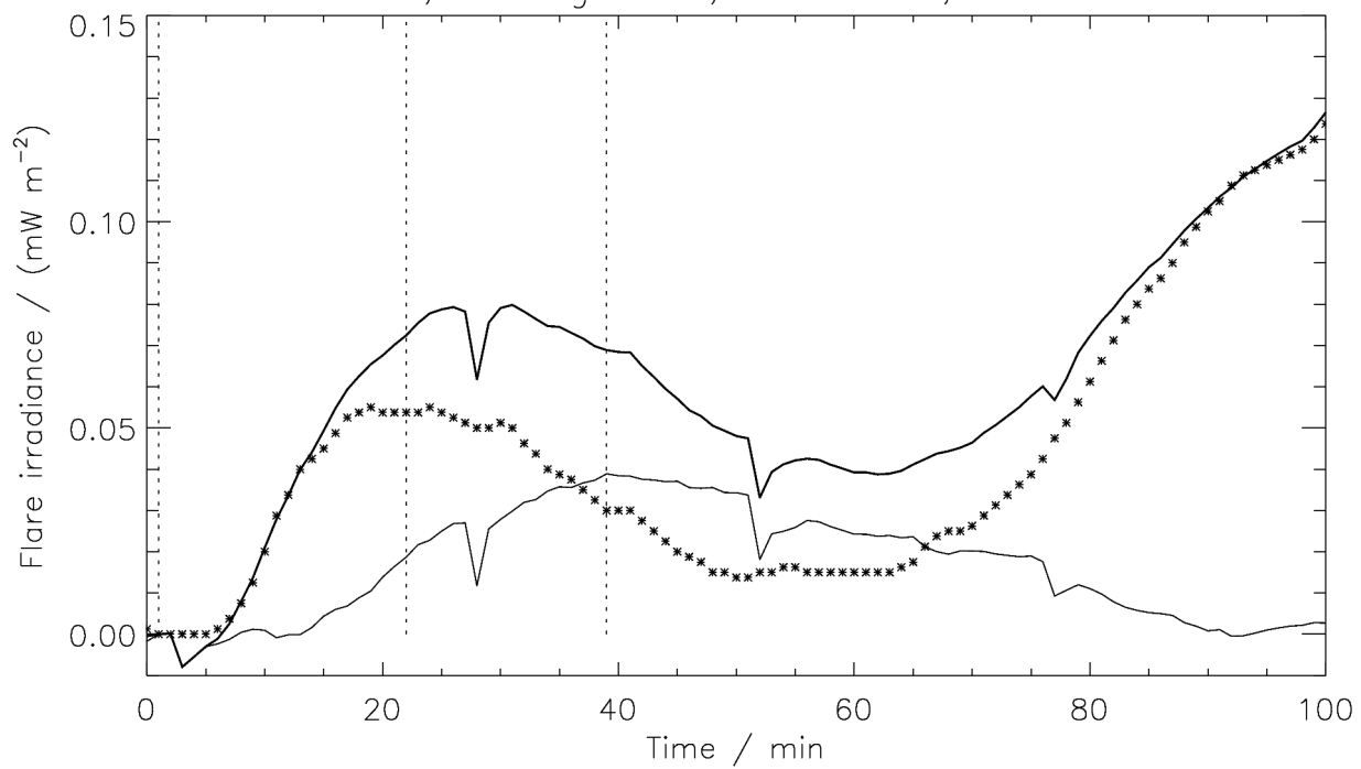
C3.5 flare, 04 Aug 2012, 15:00 UTC, ch3-125*SXR
