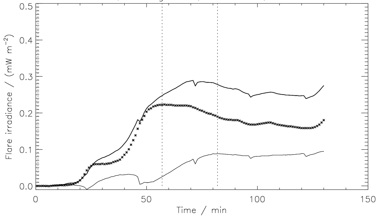
C3.5 flare, 04 Aug 2012, 15:00 UTC, ch3-95*SXR
