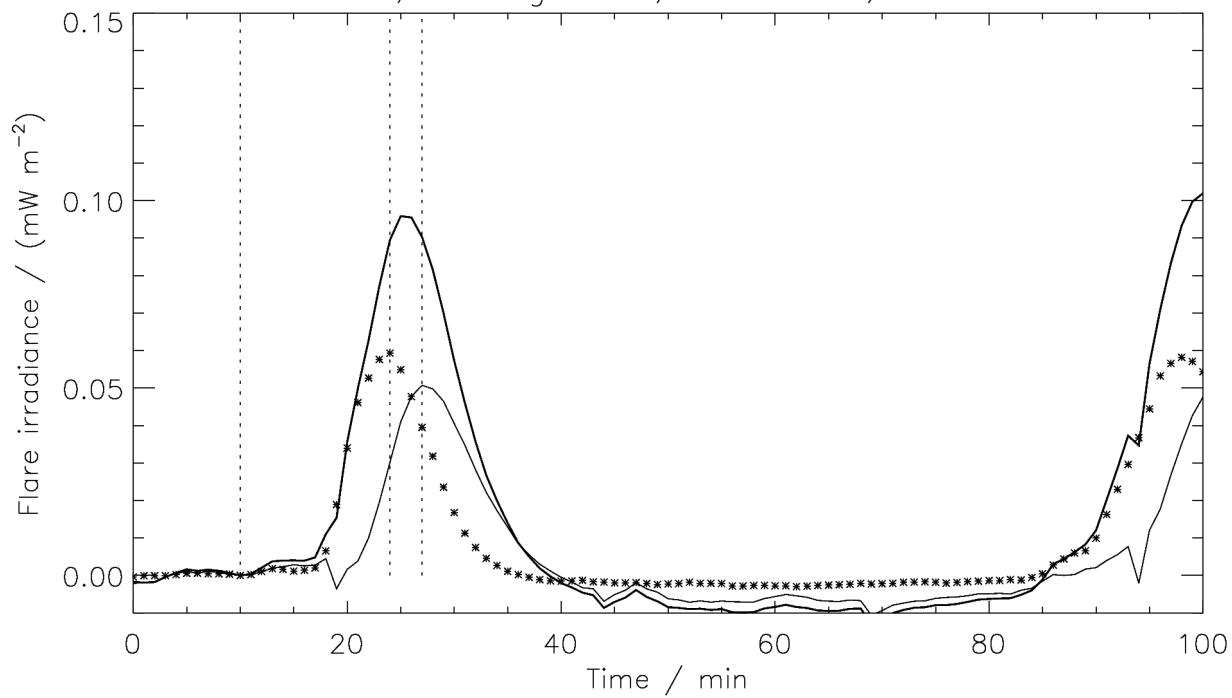
C1.7 flare, 06 Aug 2011, 10:24 UTC, ch3-55*SXR
