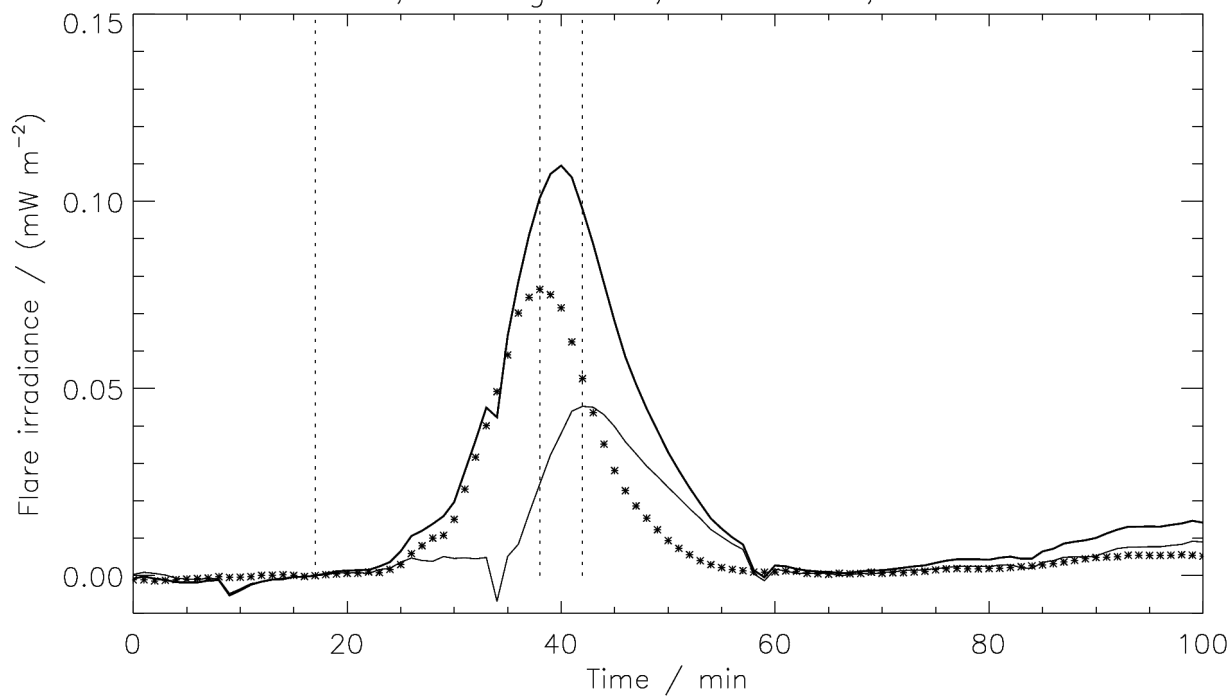
C1.6 flare, 06 Aug 2011, 11:38 UTC, ch3-70*SXR
