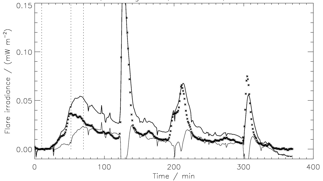
C2.8 flare, 06 Aug 2012, 16:56 UTC, ch3-150*SXR
